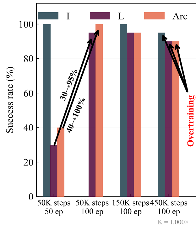
Ablation: Training configuration
